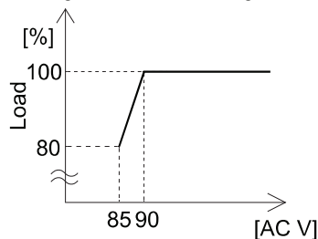
Fig.5.2 Input voltage derating curve
