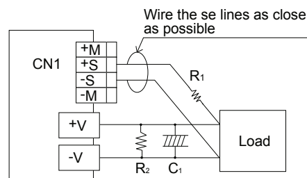
Fig.2.5 When using remote sensing function
