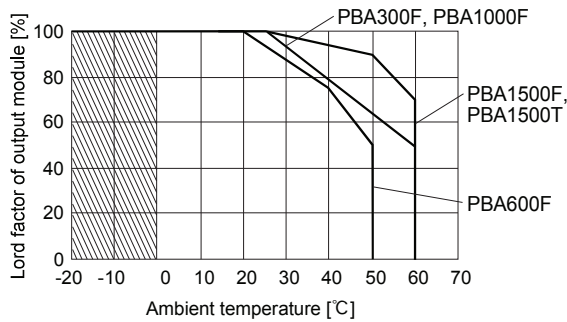
Fig.7.3 Ambient temperature derating curve (-F3)
