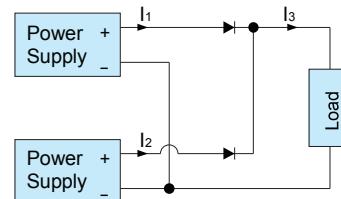
Fig.4.2 Example of connecting in redundancy operation
