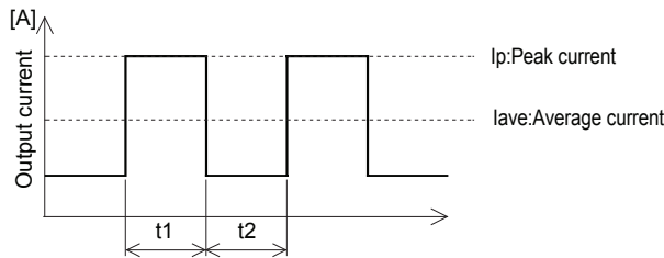
Fig.3.1 Peak current
