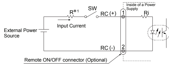
Fig.7.7 Example of using a remote ON/OFF circuit
