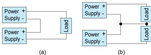
Fig.4.1 Examples of connecting in series operation
