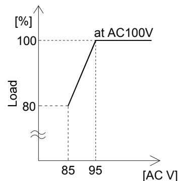
Fig.5.4 Input voltage derating curve
