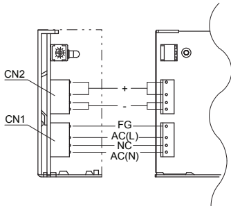
Fig.7.6 Image of option -J (PBA50F)
