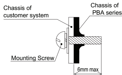
Fig.5.1 Mounting screw
